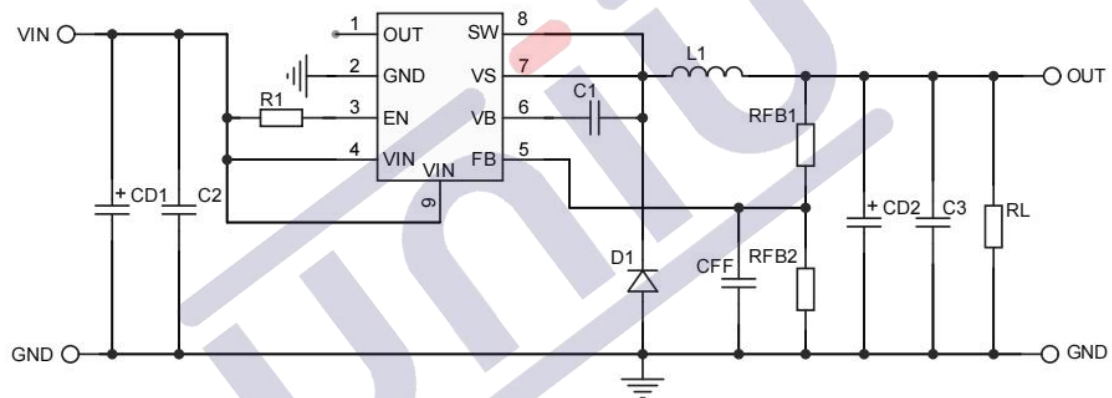
APP1: V_{OUT} < 10V
