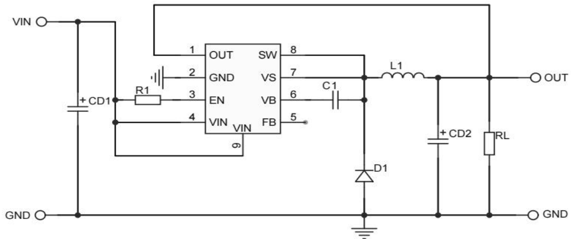
APP1: V_{OUT} < 10V
