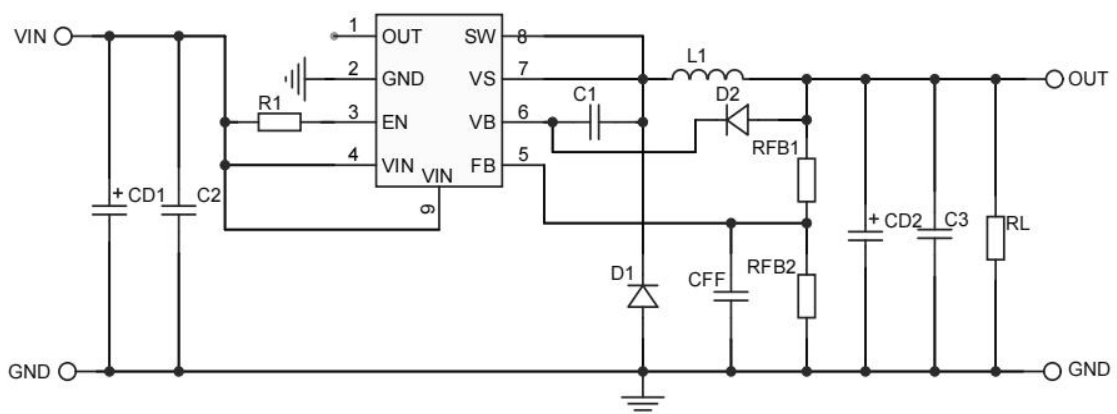
APP2: V_{OUT} = 10 \sim 15V
